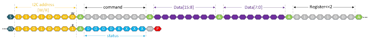
Figure 15-7. Write Register I2C Timing Diagram
