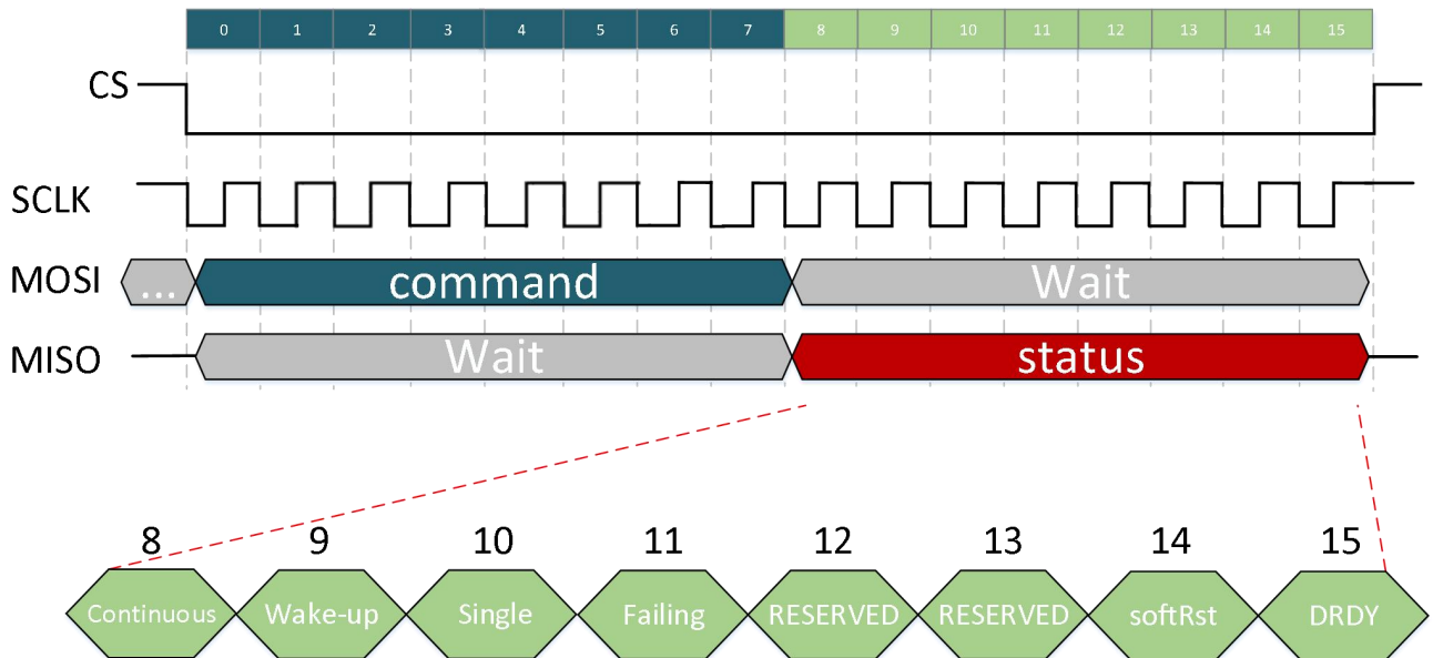
Figure 10-1. Operating Status SPI Description
