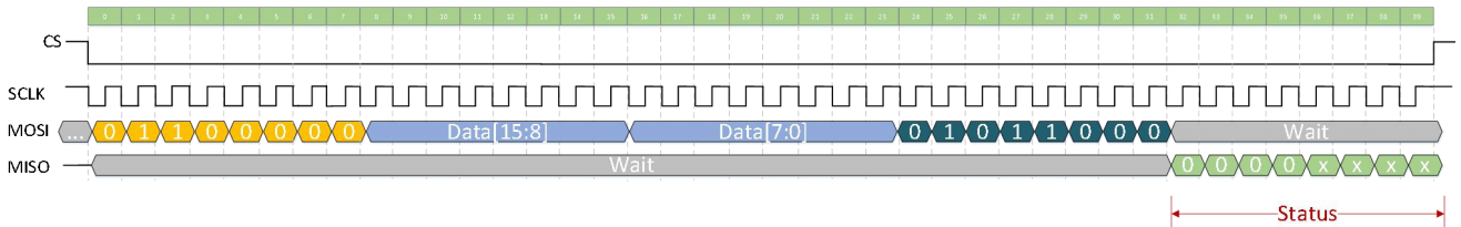
Figure 15-3. Write Register SPI Timing Diagram
