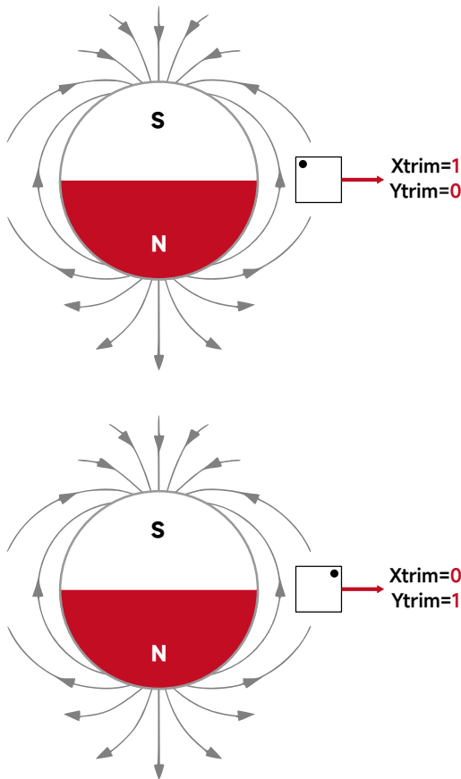
Figure 16: Illustration of Chip Placement Orientation and Setting of Xtrim and Ytrim Parameters
