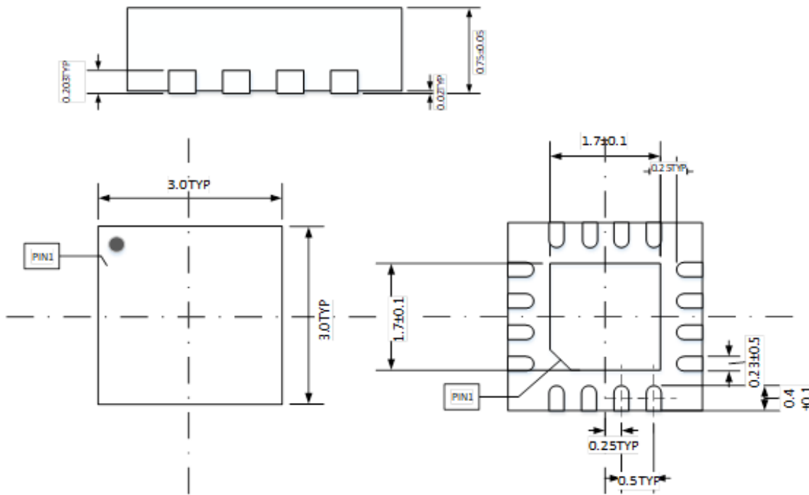
Figure 17: Packaging Information for KTH7823
