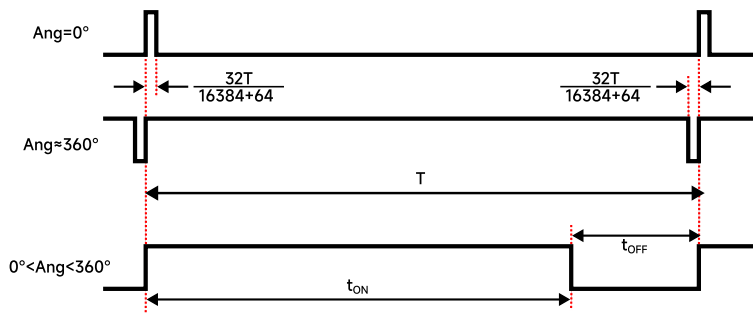
Figure 12: PWM Timing
