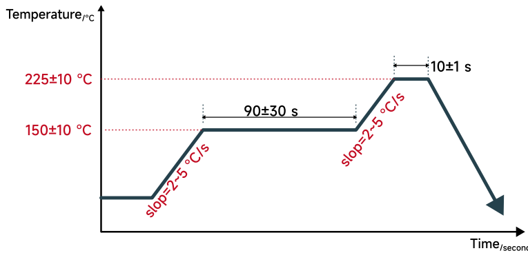
Figure 18: Soldering Temperature Profile for KTH7823
